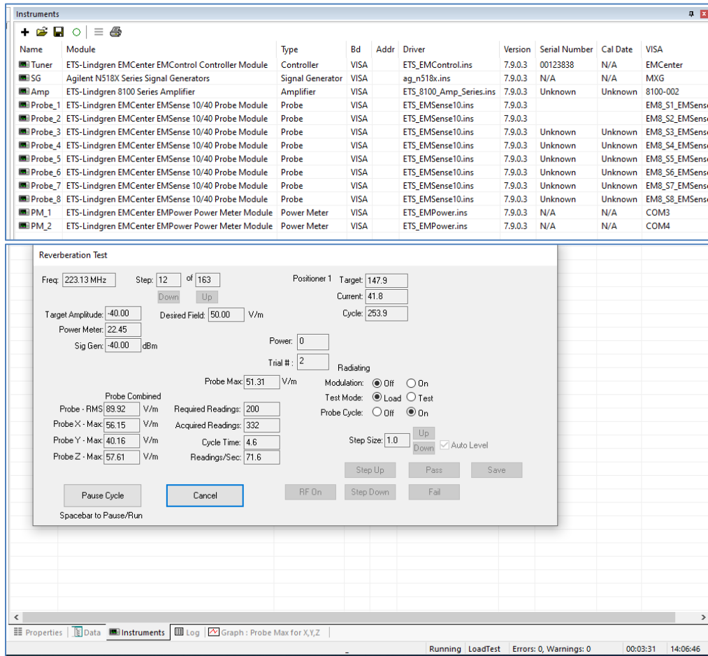
Figure 4: ISO11451-5 vehicle test of EM8 in TILE!
