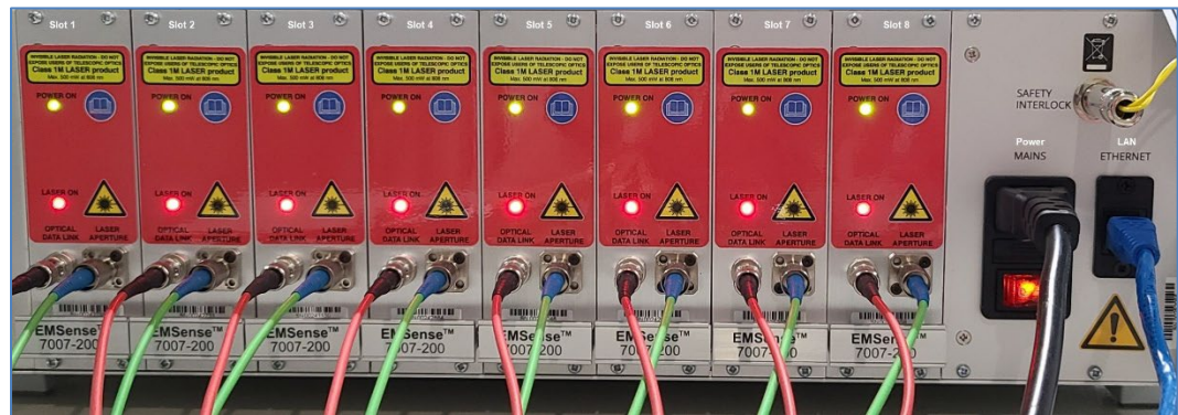
Figure 2: EM8 Back
